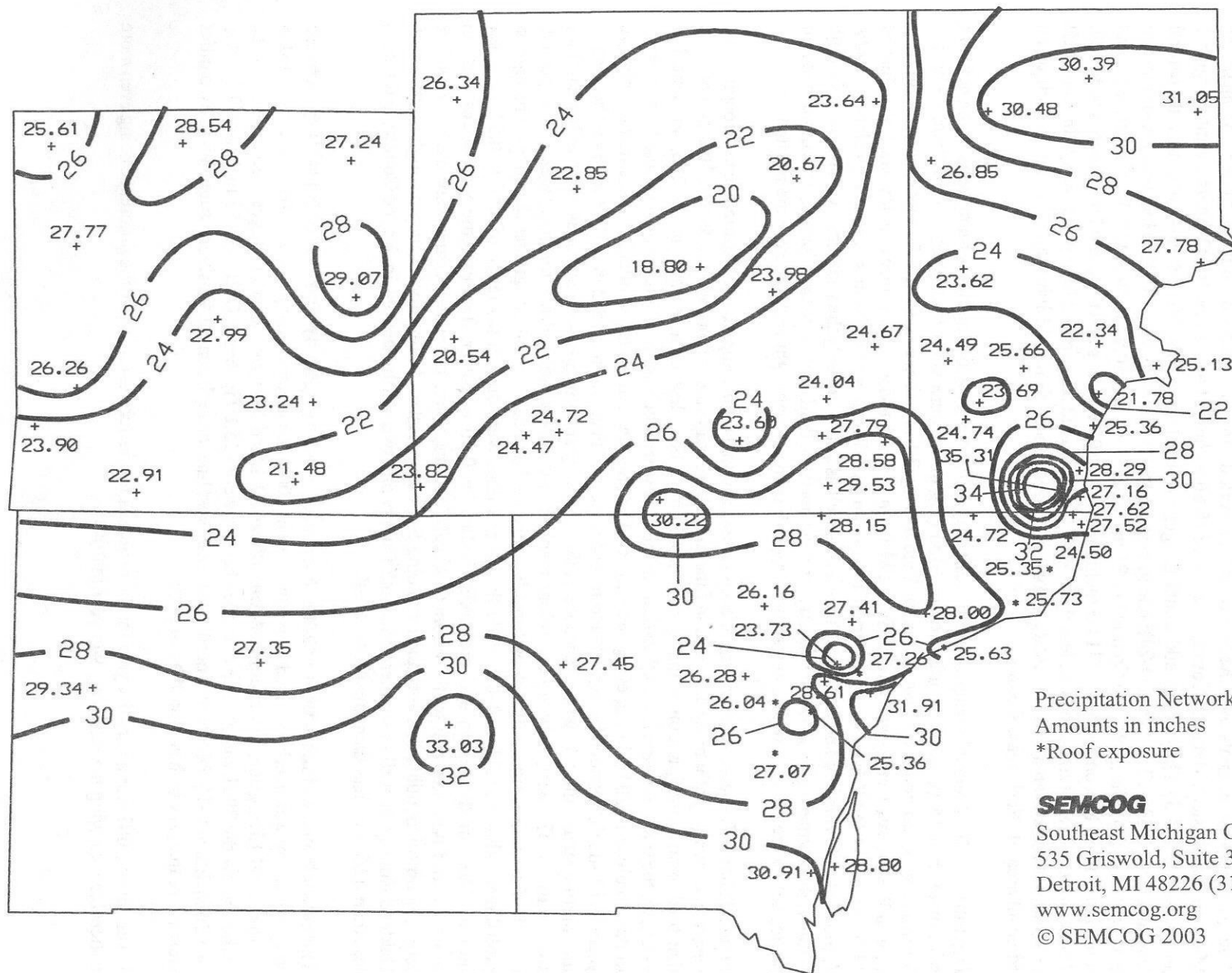
Figure 1 2002 Annual Precipitation
